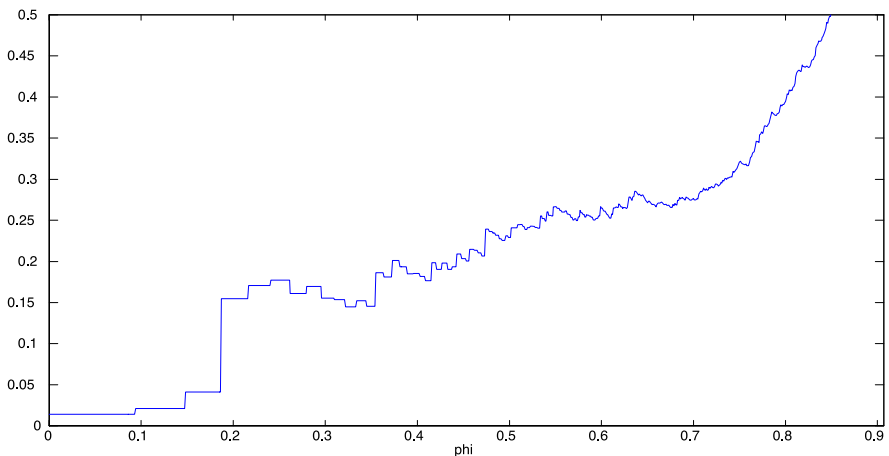
Fig. 3. Alternative Hill plot, \{(\varphi, \hat{\xi}_{\varphi,T^{\varphi}}): 0 < \varphi \leq 0.9\} , for the sample of exchange rate changes, T=1716 .
